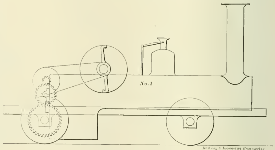
THE SWORD BLADE LOCOMOTIVE.
